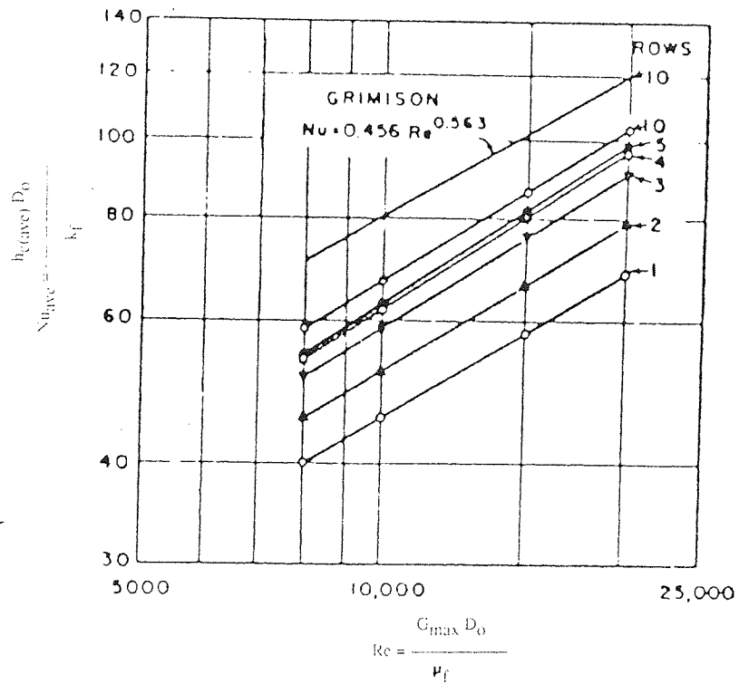
Fig. 2.8 Correlation of Nu_{av} versus Reynolds number for a ten-row tube bank (Snyder [1953])
