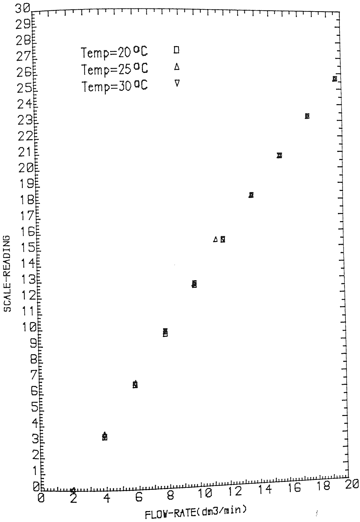
Fig. A.8 Calibration curve of Rotameter 245
