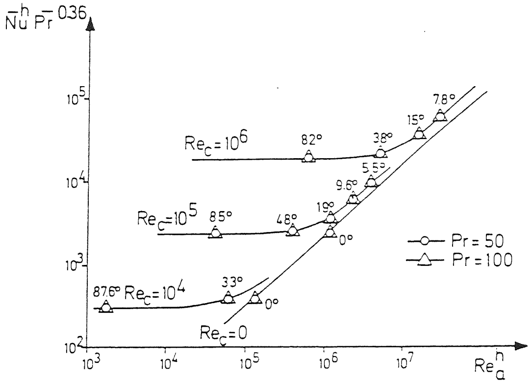
Fig. 2.5 Predicted Nu_h / Pr^{0.36} as a function of the axial Reynolds number Re_a with the transverse Reynolds number Re_c as a parameter for fully-developed inclined flow through a staggered arrangement of P_t \times P_l = 2.42 \times 1.64 (Antonopoulos [1985])
