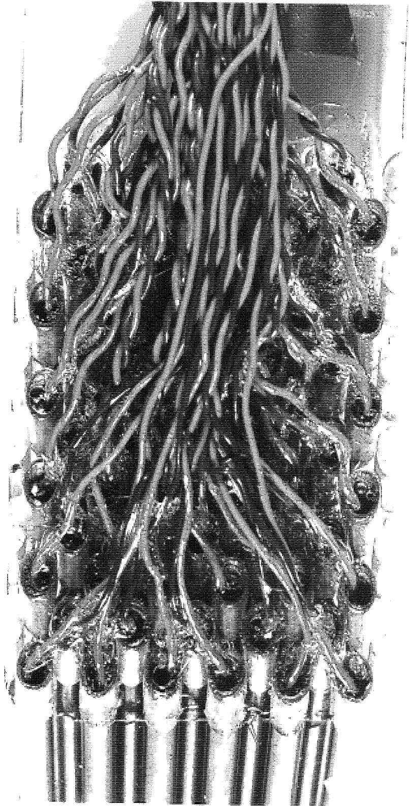
Fig. 6.5b Photograph of the inclined tube bank ( \phi=57.5^\circ )
