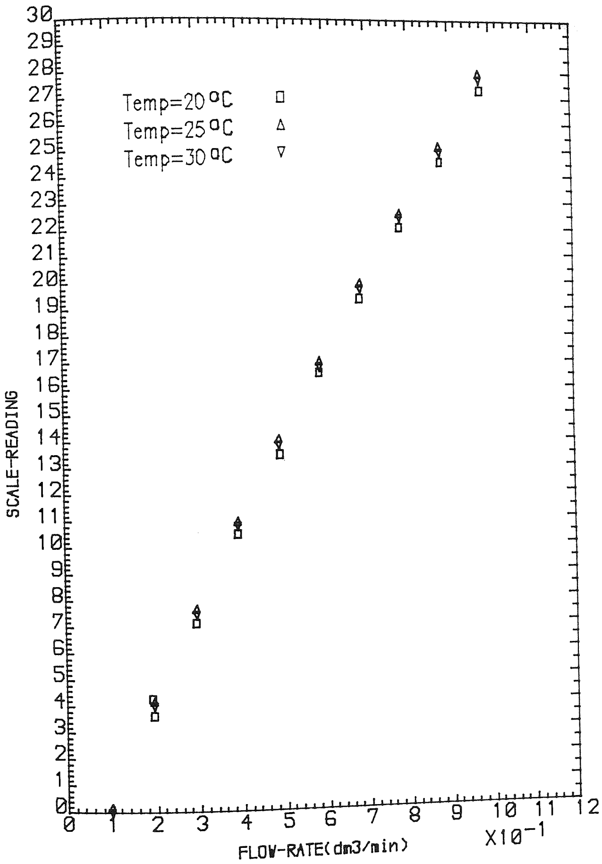
Fig. A.3 Calibration curve of Rotameter 7S
