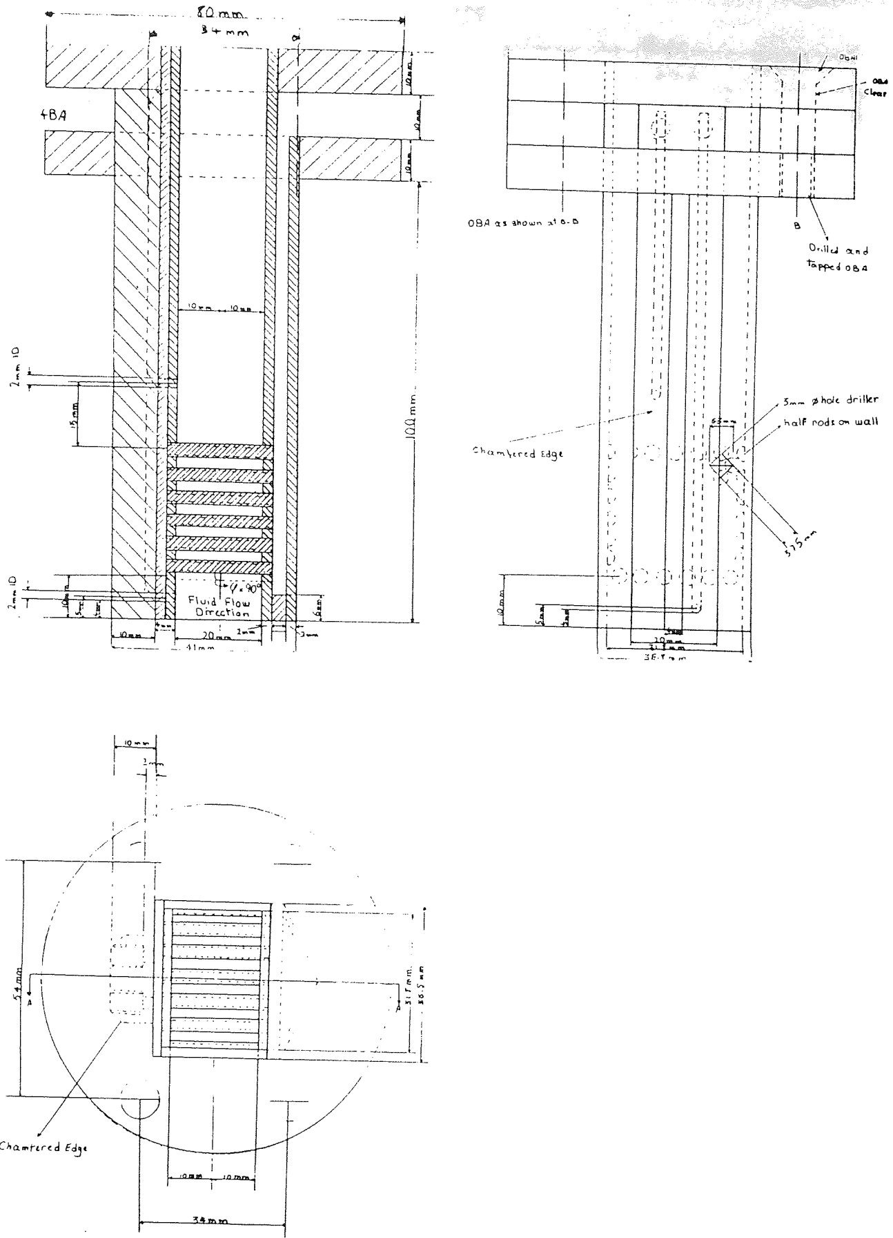
Fig. 6.6 Full drawing of first model
