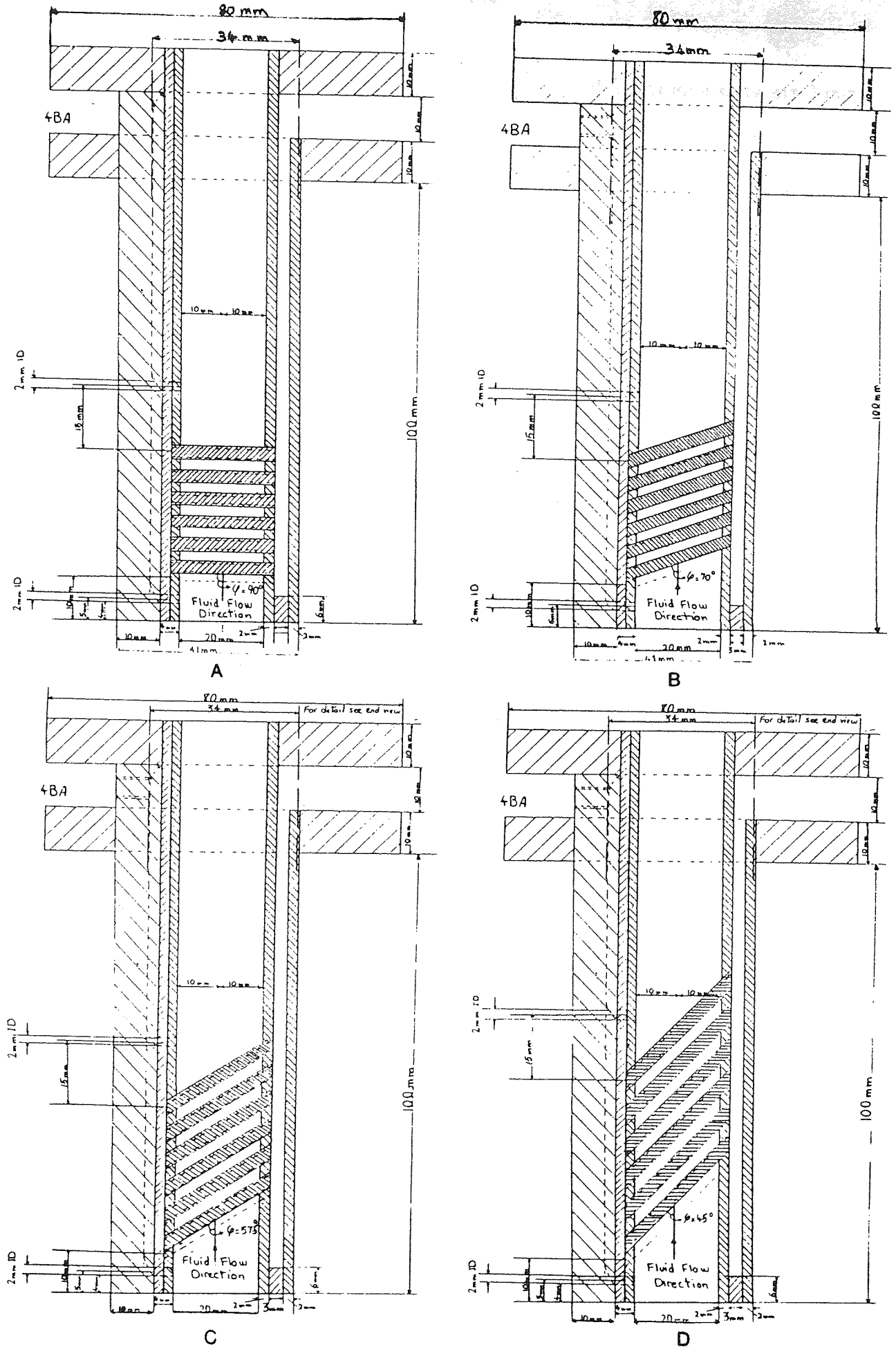
Fig. 6.7 Cross section drawing of four models
