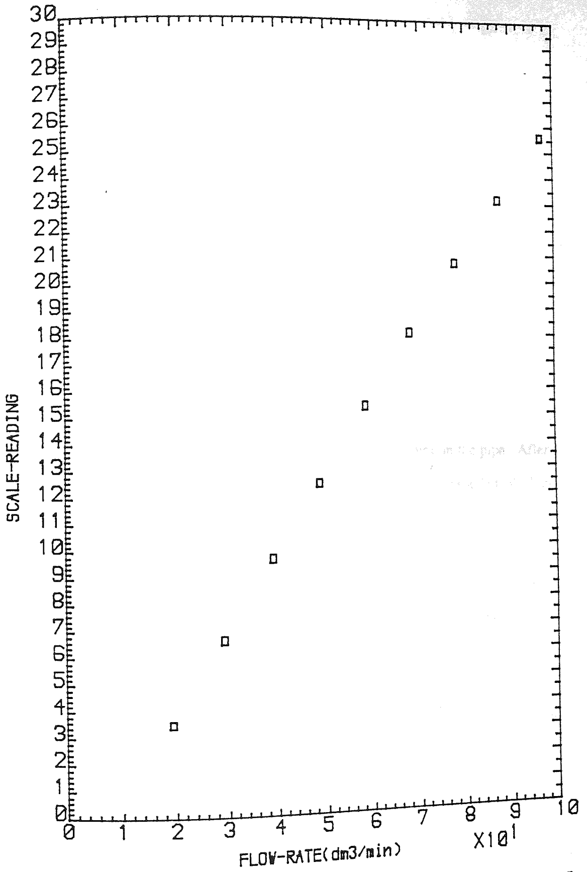
Fig. A.10 Calibration curve of Rotaneter 47S Temp=25°C
