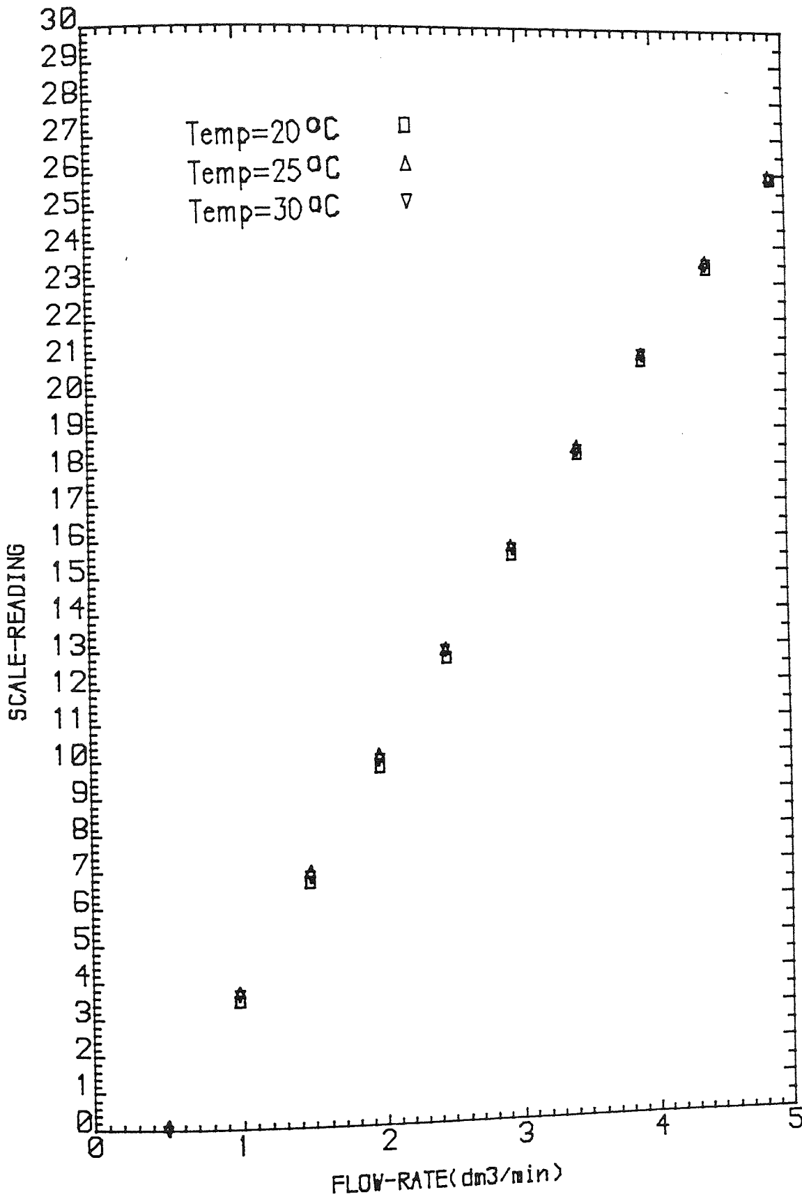
Fig. A.6 Calibration curve of Rotameter 145
