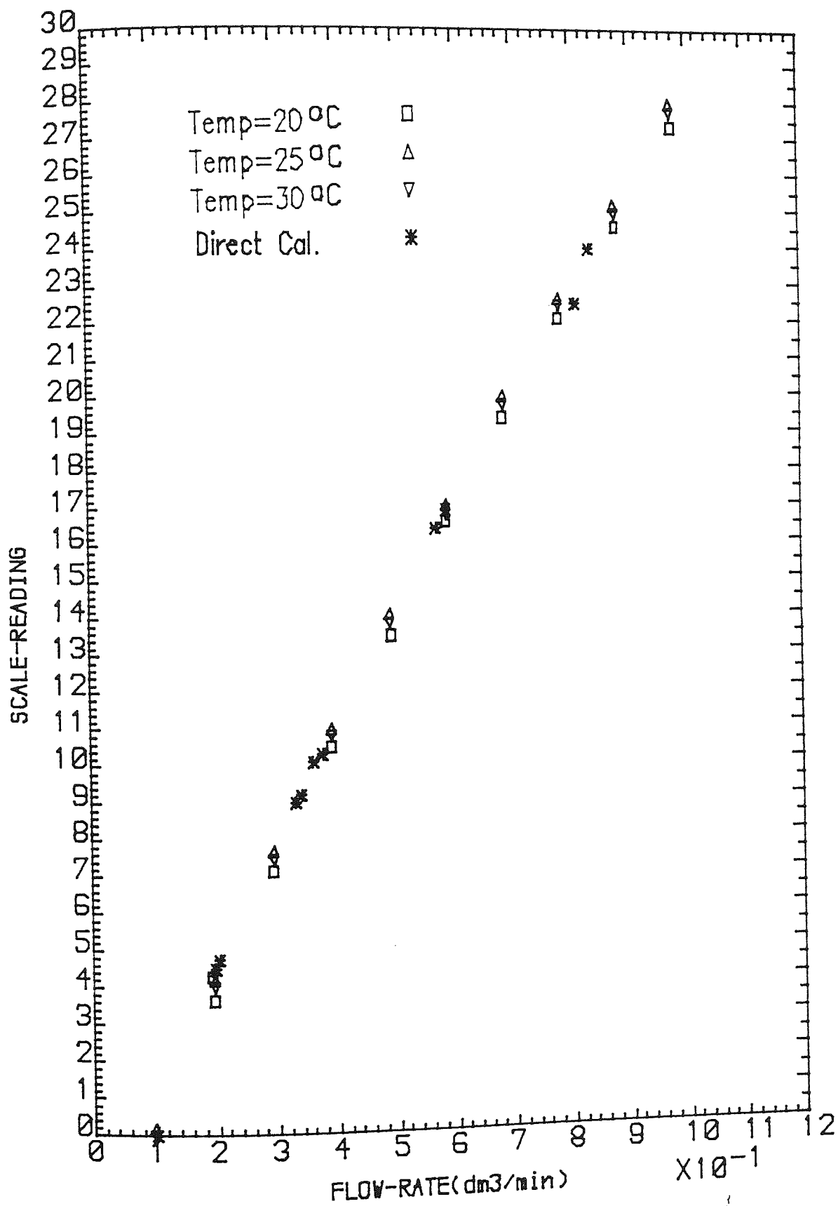
Fig. A.4 Comparison of two calibration methods
