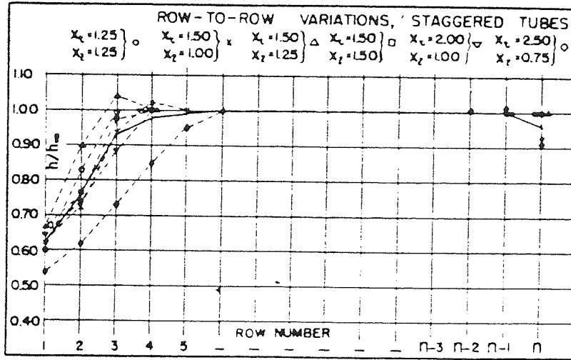
Fig. 2.9 Row-to-row variation of normalised heat transfer coefficient (Kays et al. [1954])
