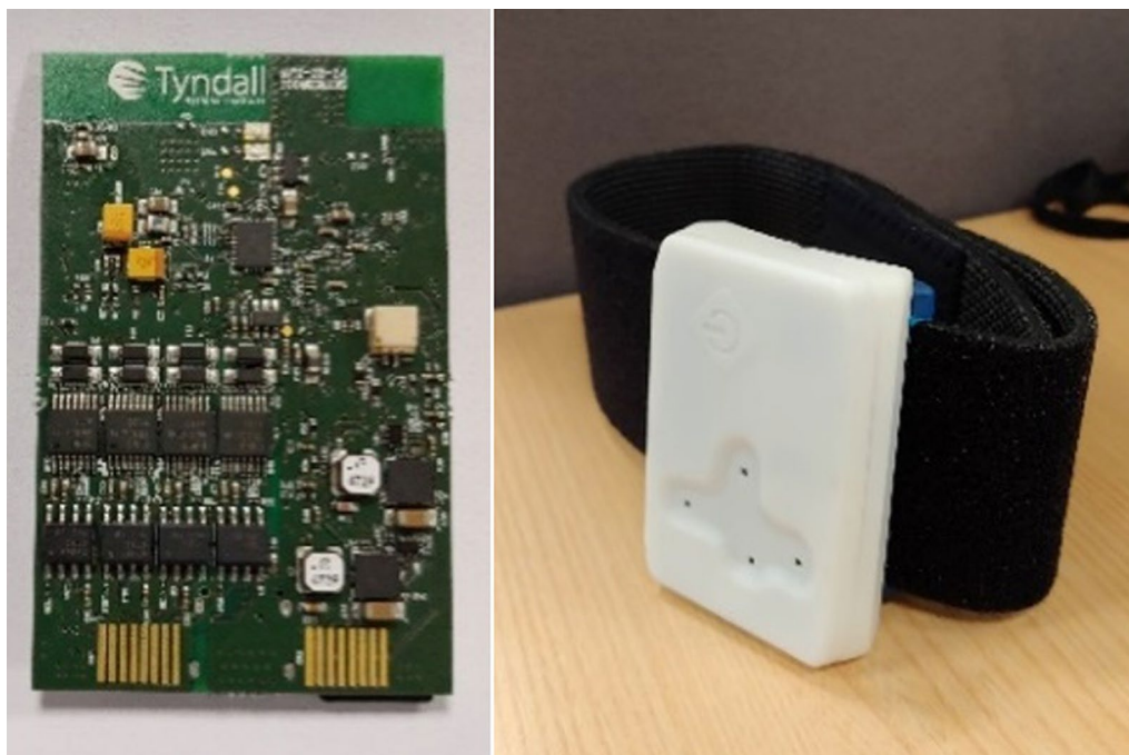
Fig. 1 PCB board (left) and 3D printed enclosed device with Velcro strap (right)
